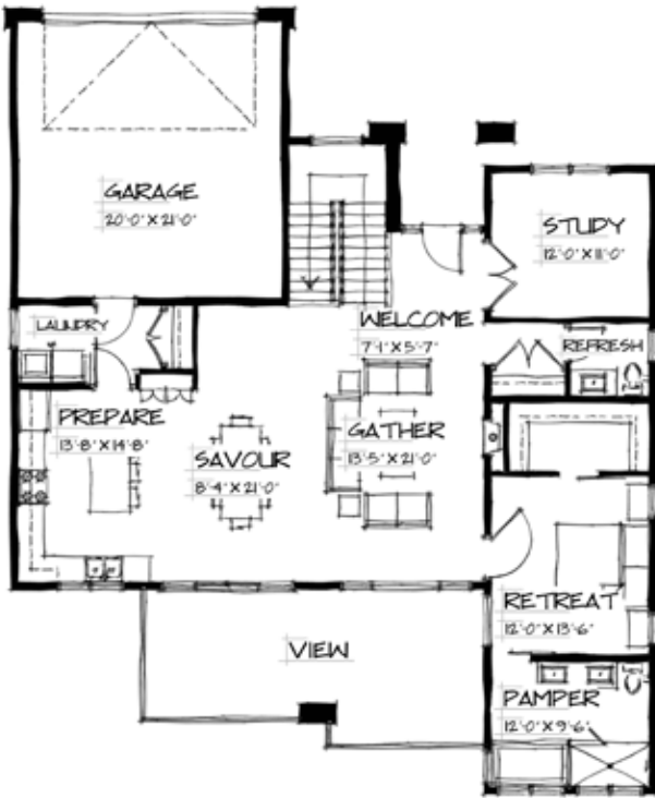
MAIN FLOOR PLAN 1561 SQ. FT. + DOUBLE GARAGE
