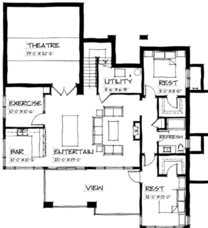
LOWER FLOOR PLAN 2009 SQ. FT.
