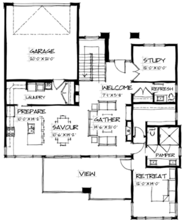
MAIN FLOOR PLAN 1595 SQ. FT. + DOUBLE GARAGE
