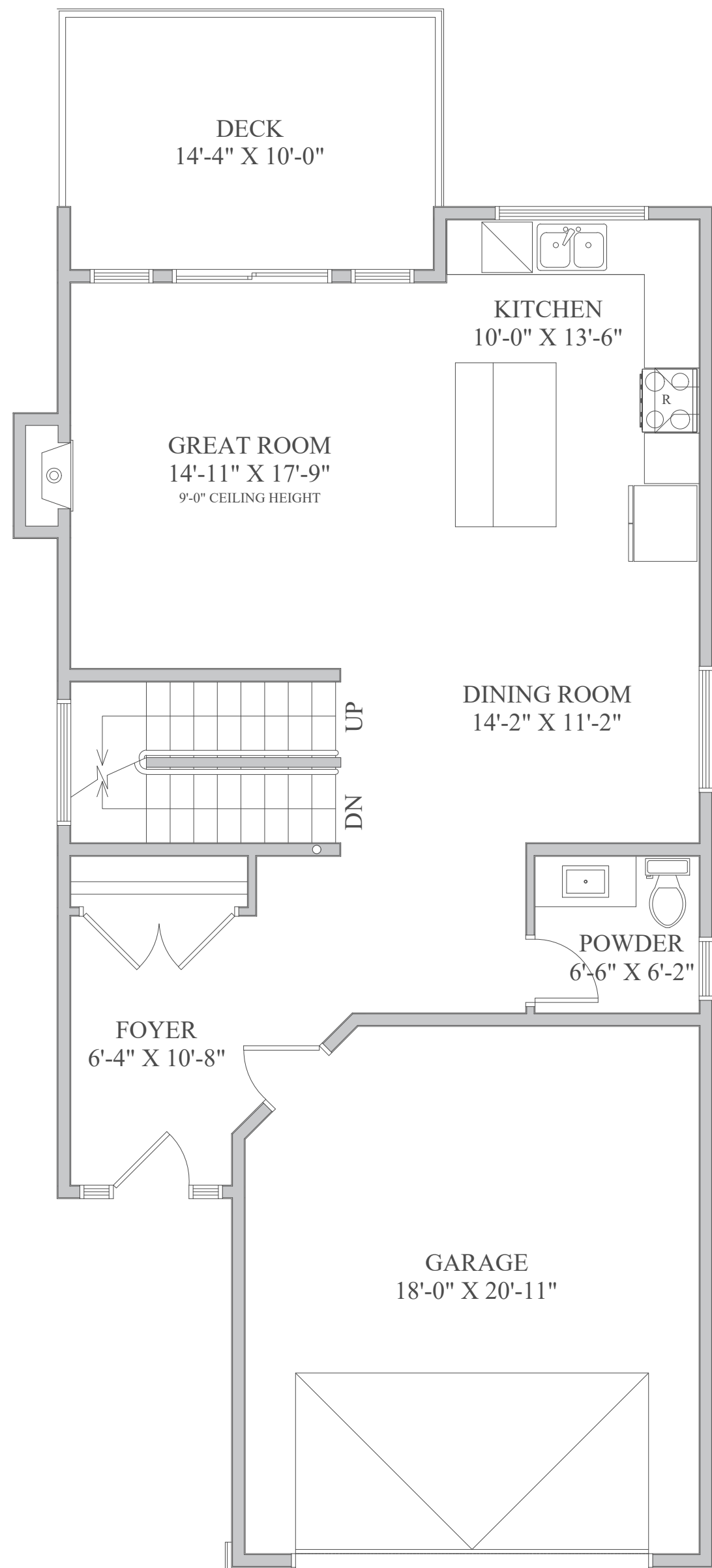
MAIN FLOOR PLAN 803 SQ. FT. + DOUBLE GARAGE
