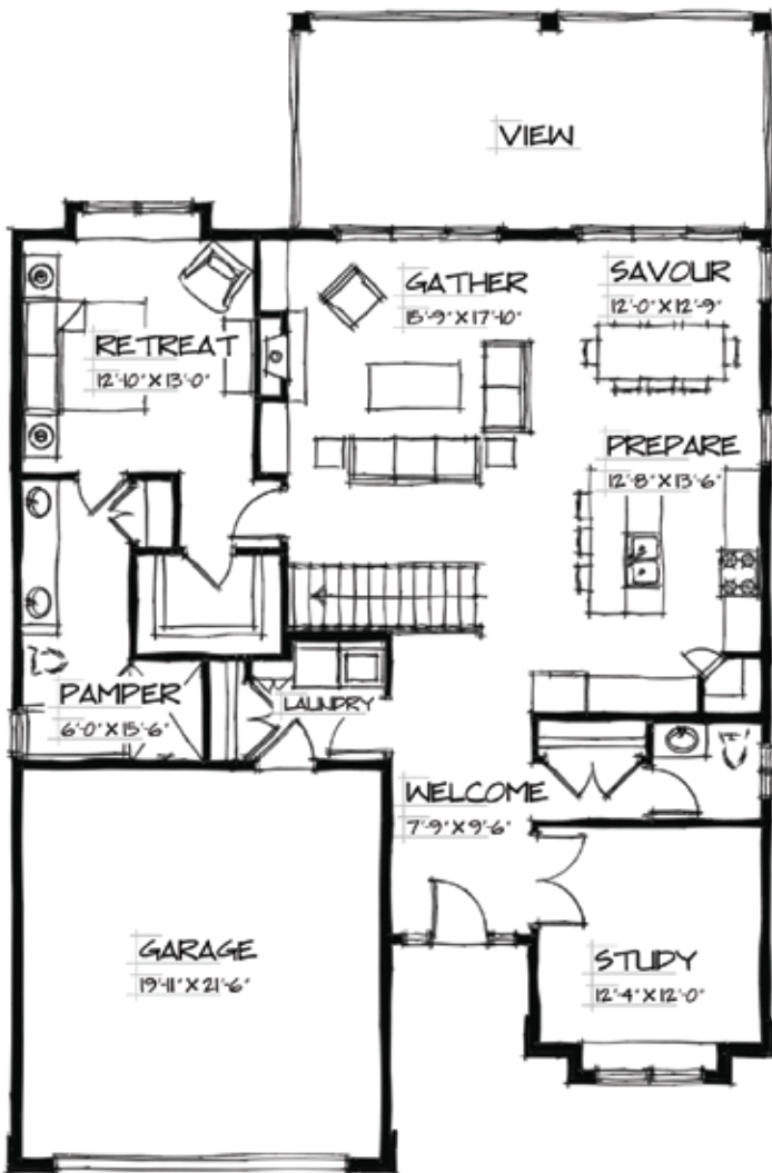
MAIN FLOOR PLAN - OPTIONAL PANTRY 1545 SQ. FT. + DOUBLE GARAGE
